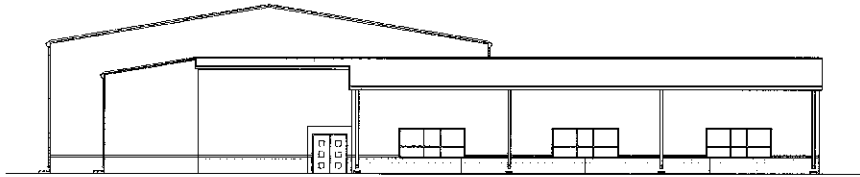
WEST ELEVATION SCALE 1/8" = 1'-0"
